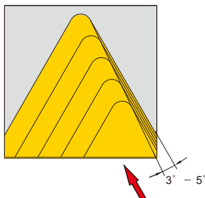
沿齿侧面进刀改进型 Cutting along teeth side with angle
